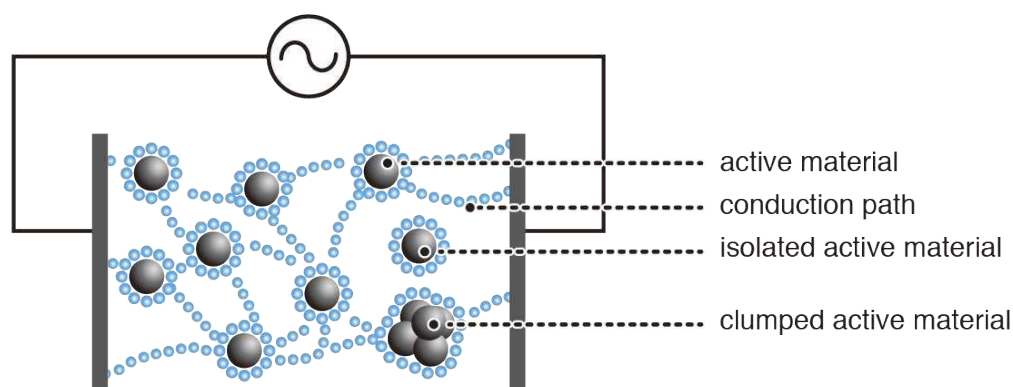
Figure 3. Measuring the impedance of an electrode slurry
