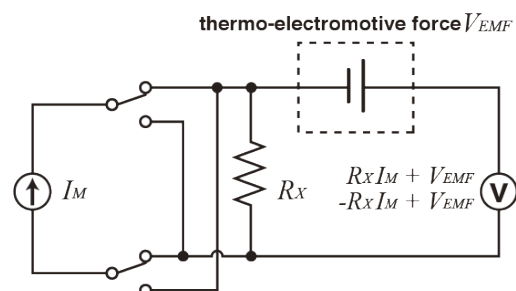
Figure 12. Cancellation of thermal electromotive force using the OVC function
