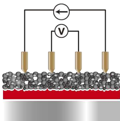
Figure 5. Measurement using the 4-probe method
