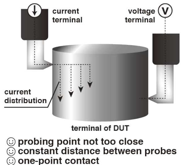
Figure 35. Reproducible contact method
