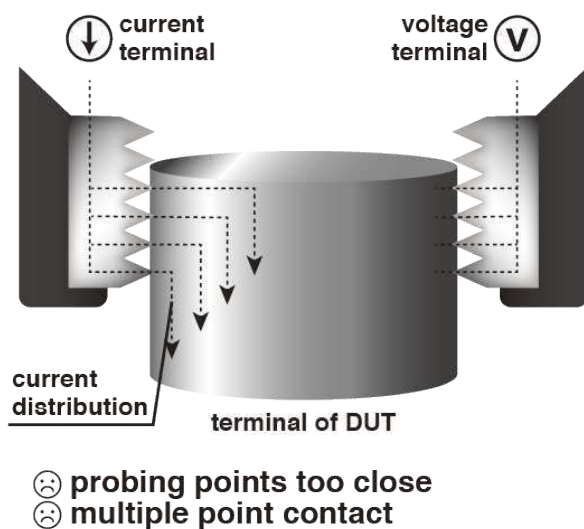
Figure 34. Influence of multi-point contact
