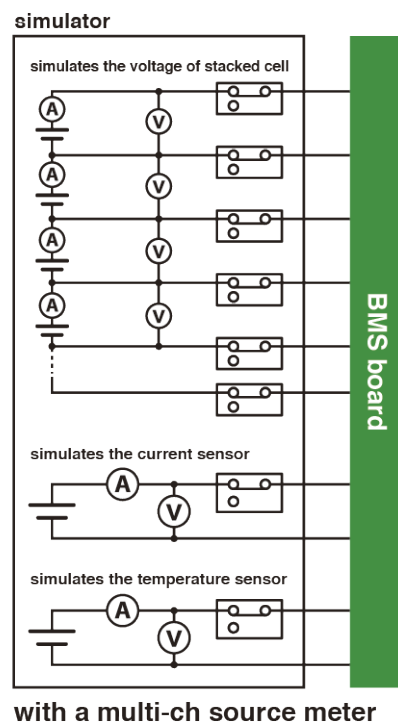
Figure 45. Example architecture of a simulation system
