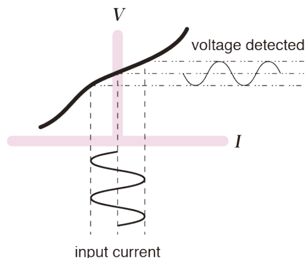
Figure 32. Detected voltage when the measurement current is appropriate
