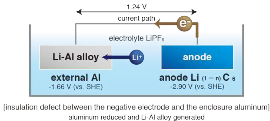
Figure 18. A reaction caused by an insulation defect between the negative electrode and the enclosure aluminum
