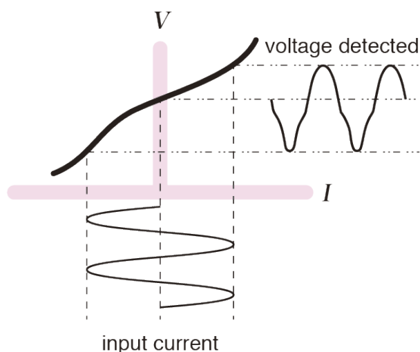
Figure 31. Distortion in the detected voltage when the measurement current is too large
