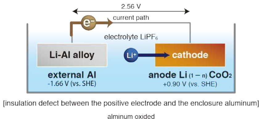
Figure 19. A reaction caused by an insulation defect between the positive electrode and the enclosure aluminum
