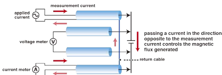
Figure 30. Four-terminal-pair method
