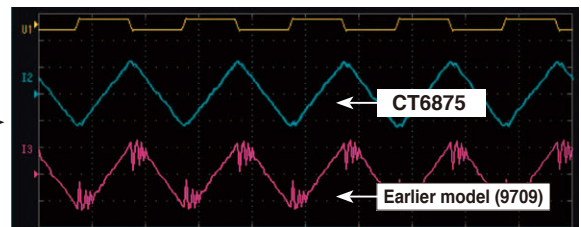
Comparison of measurement waveforms, CT6875 and Earlier model
