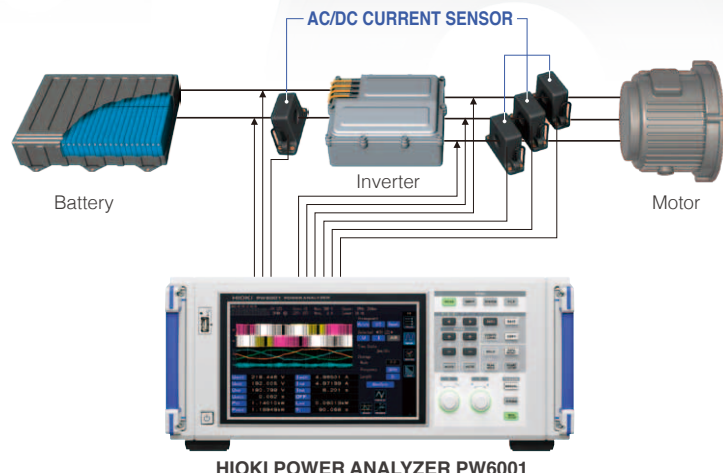
HIOKI POWER ANALYZER PW6001
