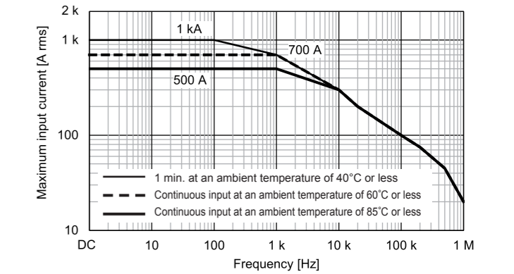
Figure 1. Frequency Derating Curve
