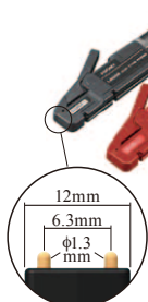
CLIP TYPE PROBE L2002 Cable length 1.5 m (4.92 ft)
