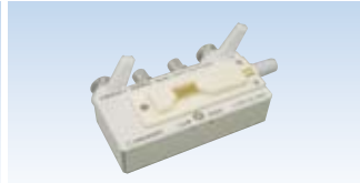
SMD TEST FIXTURE 9263 DC to 5 MHz Test sample dimensions: 1 to 10 mm
