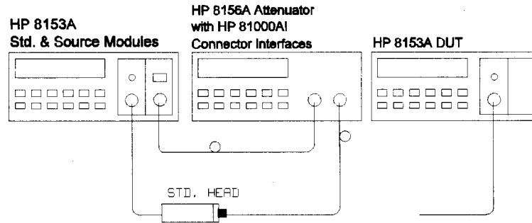
Figure D-1. Accuracy and Linearity Test Setup
