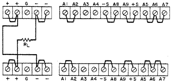
Figure 3-9. Normal Series Operation
