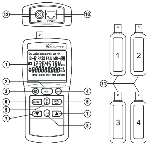
Fig. 2: Instrument and remote identifiers #1 ~ #4
