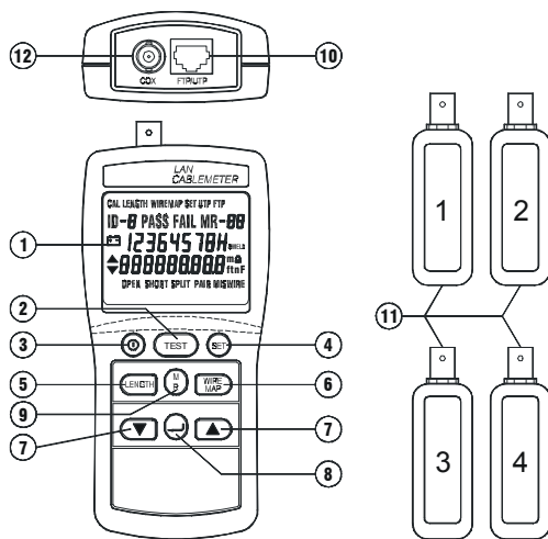
Fig. 2: Instrument and remote identifiers #1 ~ #4
