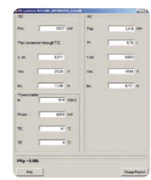
Photovoltaic testing result on PC application TOPVIEW.
