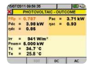
Photovoltaic testing result.
