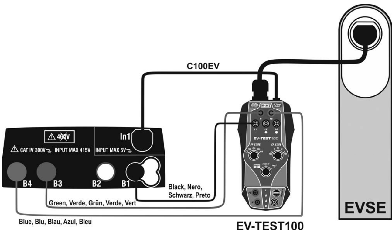
Fig. 2: Use of the adapter for testing EVSE
