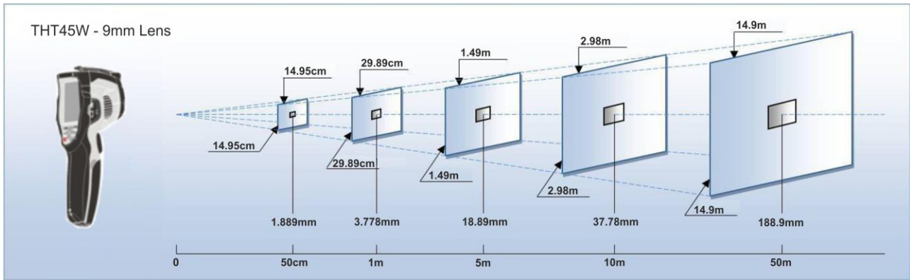
Fig. 36: Representation of the THT45 or THT45W instrument's D/S ratio
