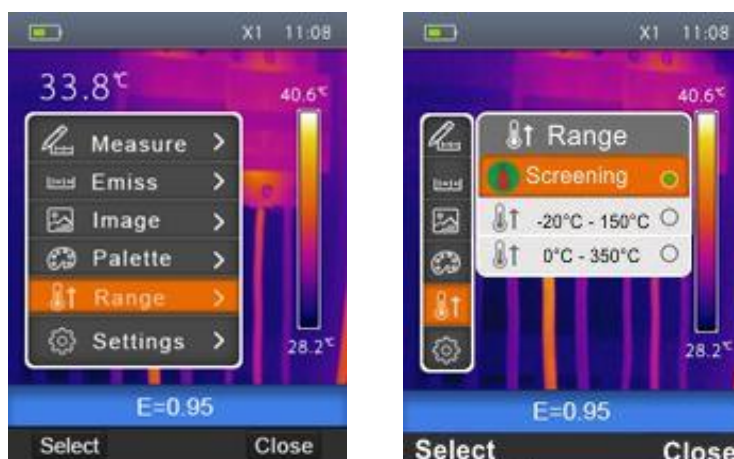
Fig. 27: Setting measuring range on the instrument
