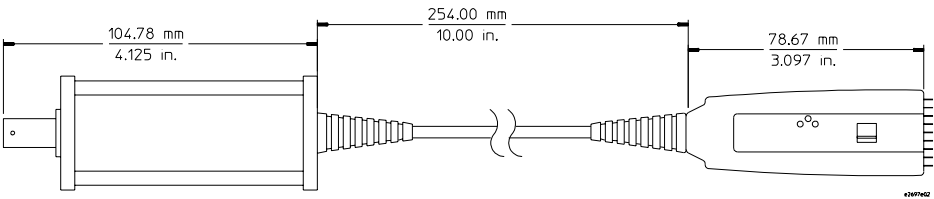
E2697A 1 MΩ Impedance Adapter Dimensions
