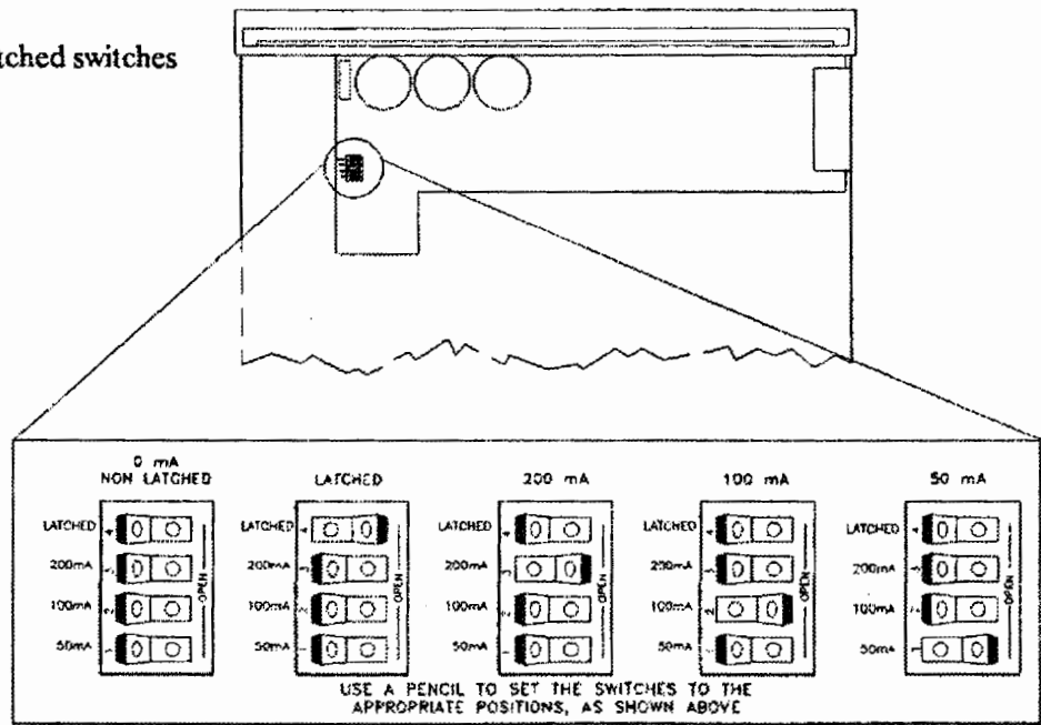
Figure D-2. Selecting Battery Options
