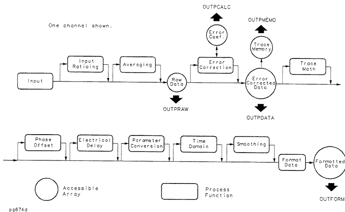
Figure 1-1. Data Processing Chain
