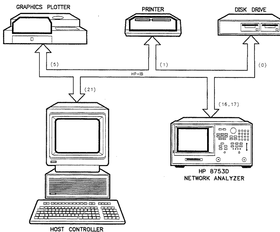
Figure 2-2. Analyzer Single Bus Concept
