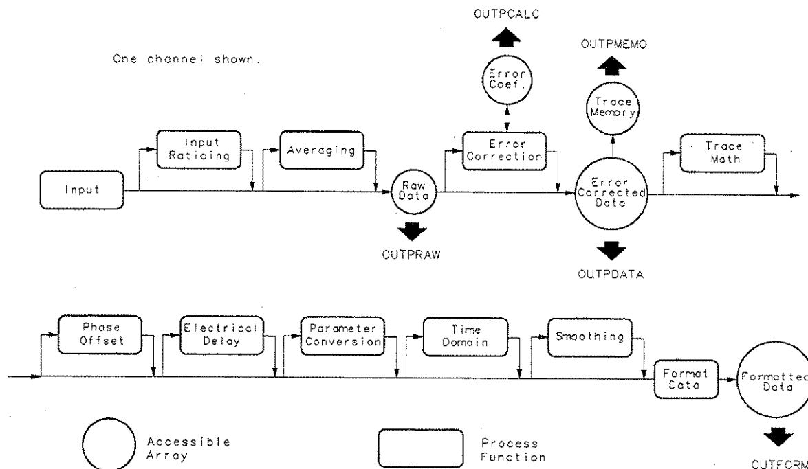
Figure 2-3. The Data-Processing Chain
