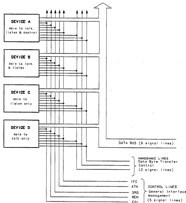
Figure 2-1. HP-IB Bus Structure
