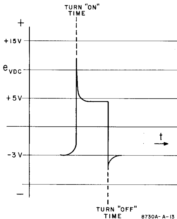
Figure 14. Dynamic Bias Switching Waveform
