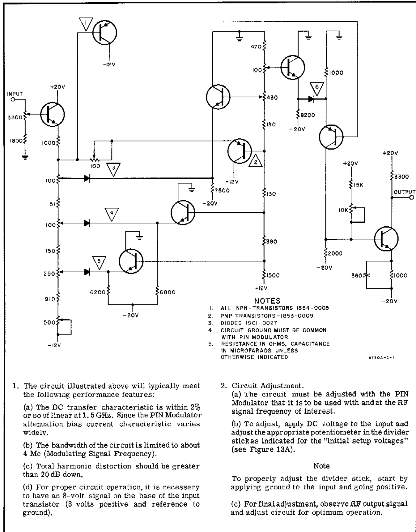
Figure 13B. Typical Shaping Circuit
