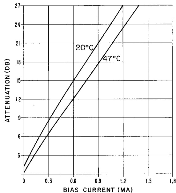
Figure 8. Typical Attenuation Variation at two Different Ambient Temperatures
