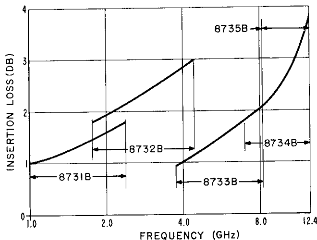
Figure 4. Typical Insertion Loss Curves
