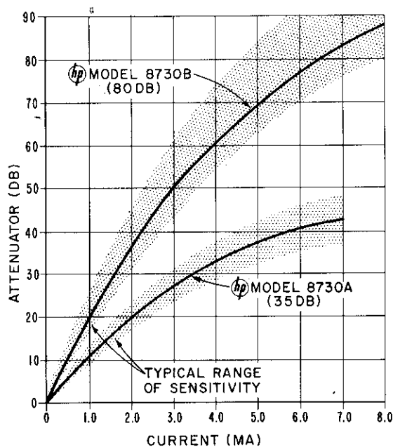
Figure 5. Typical Sensitivity (Plotted with frequency constant)
