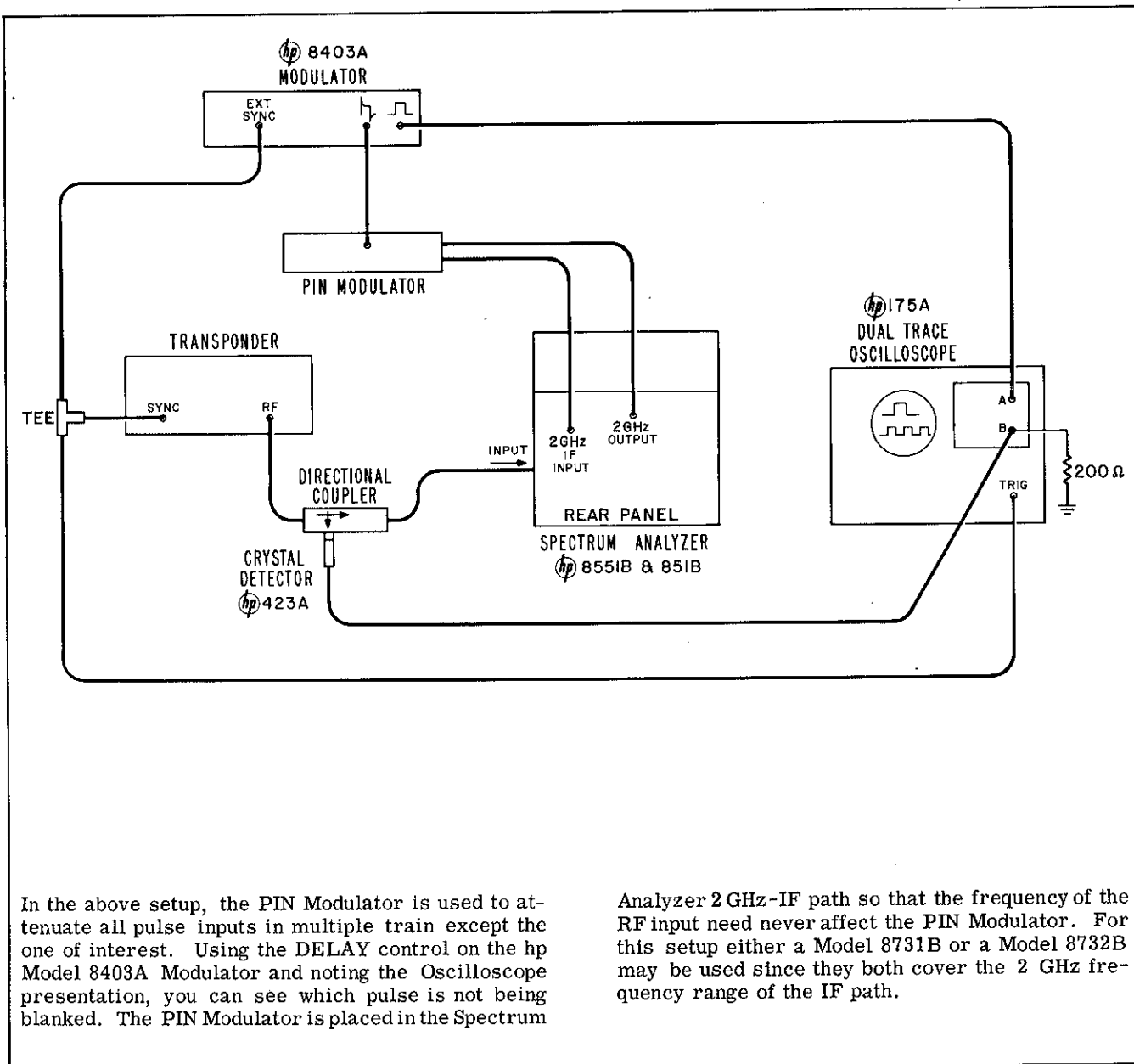
Figure 16. Multiple Signal Separation for Spectrum Analysis
