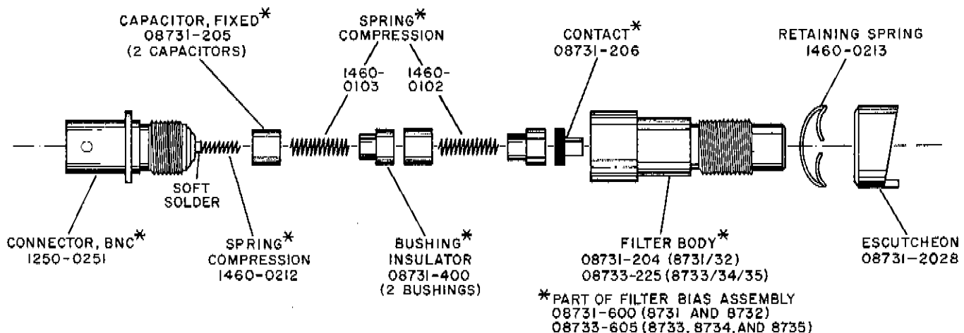
Figure 18. Bias Input Assembly
