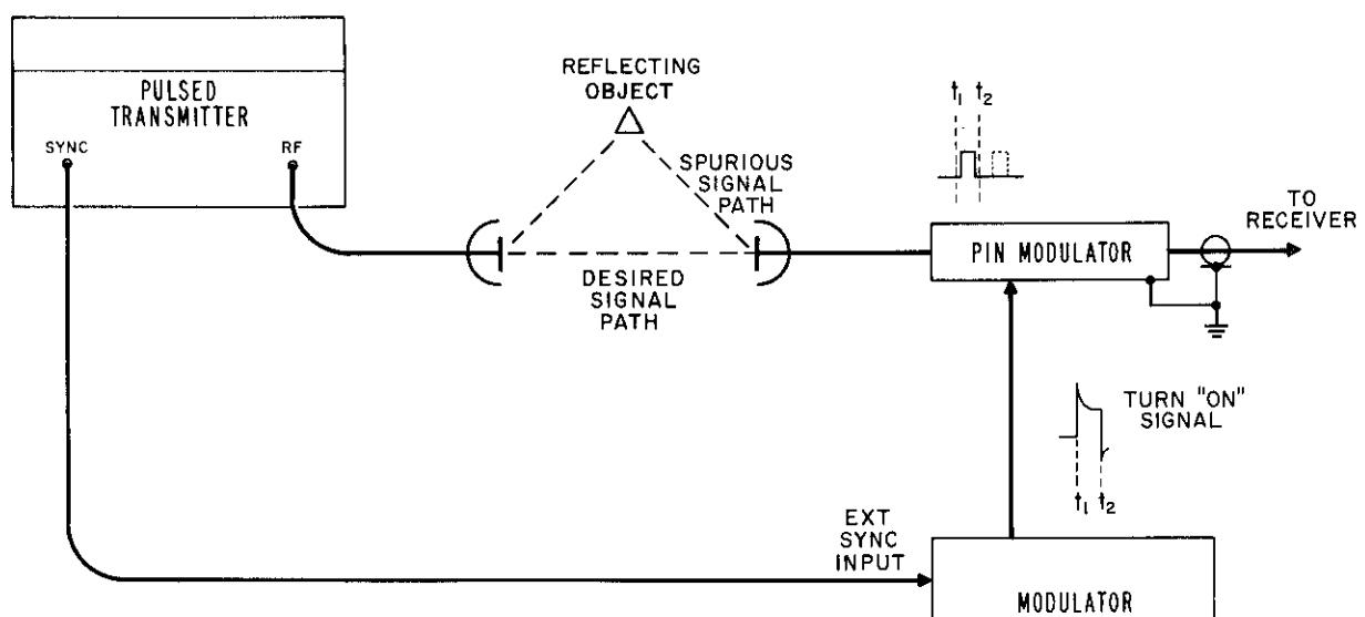
Figure 15. Typical Use of PIN Modulator as an RF Gating Device
