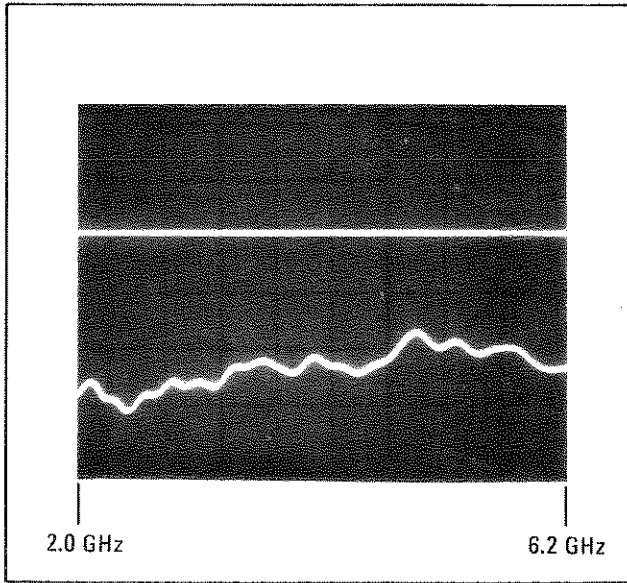
Figure 3-5. Unlevelled RF Power Output
