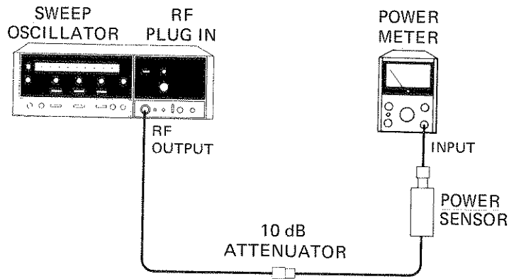
Figure 2-4. Internal Leveling Test Setup
