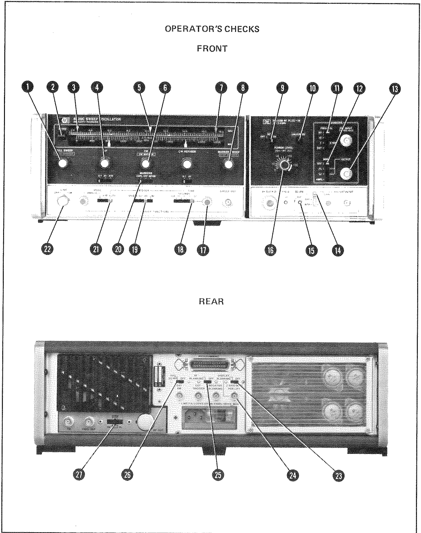
Figure 3-3. Operator's Checks (1 of 3)
