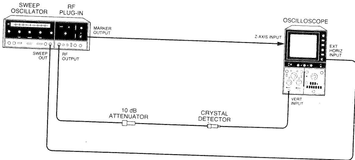
Figure 2-6. Marker Range Test Setup
