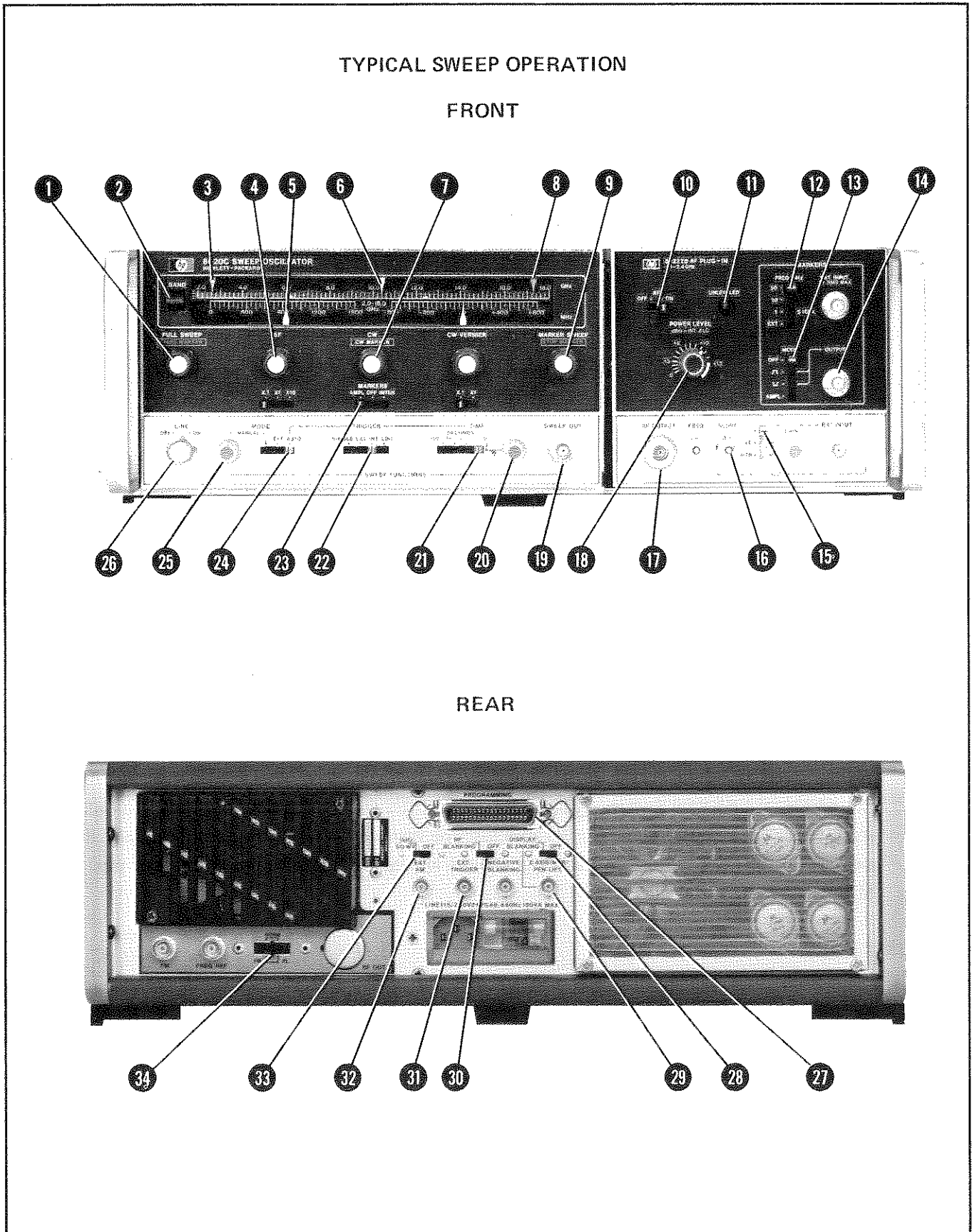
Figure 3-4. Typical Sweep Operation (1 of 5)
