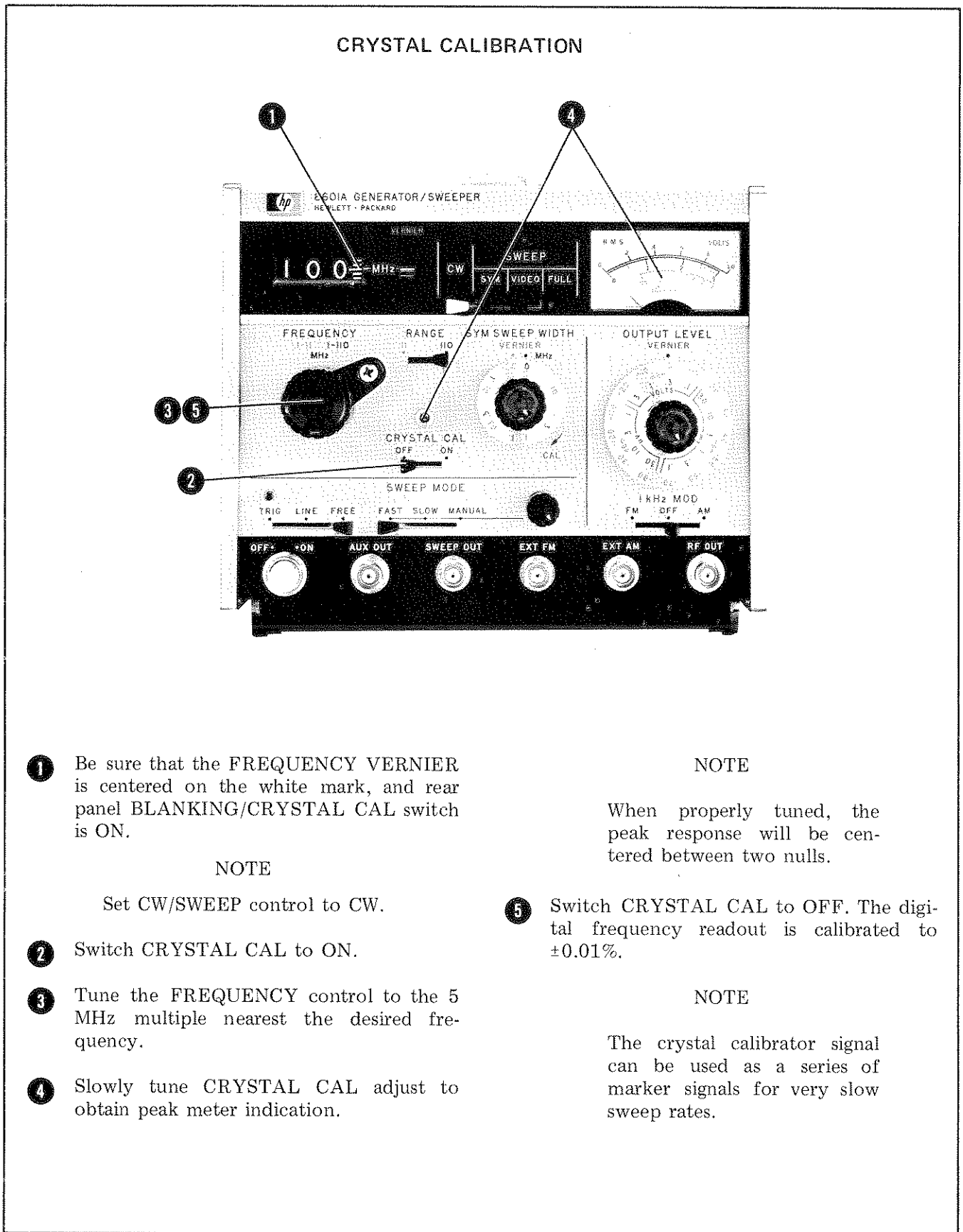
Figure 3-5. Crystal Calibration
