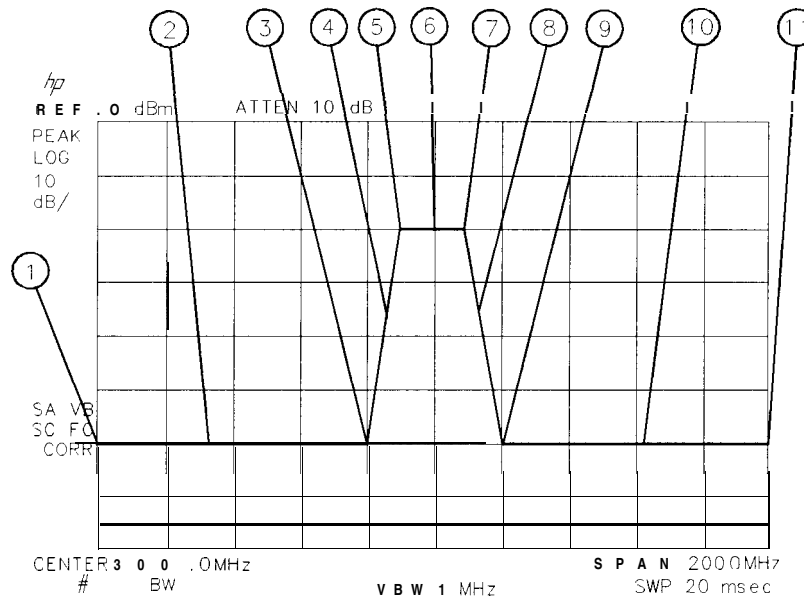
Figure 5-6. Limit-Line Segments
