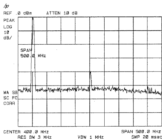
Figure 3-21. Harmonic Distortion
