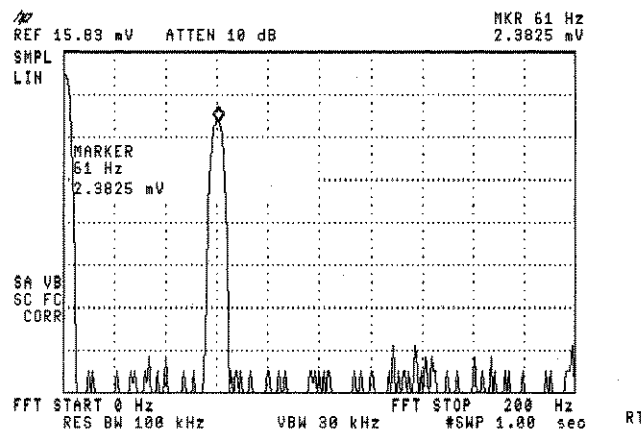
Figure 4-1. FFT Annotation
