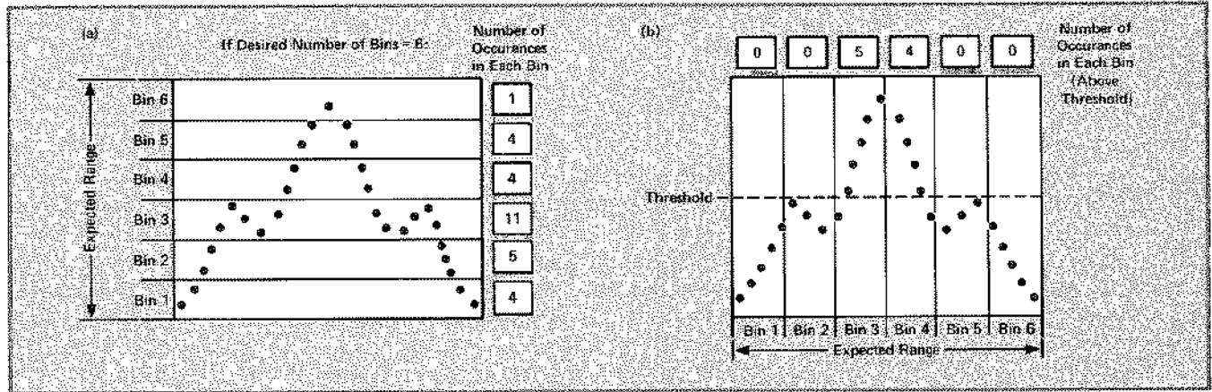
Figure 2. (a) Probability Distribution of y-axis. (b) Probability Distribution of x-axis.
