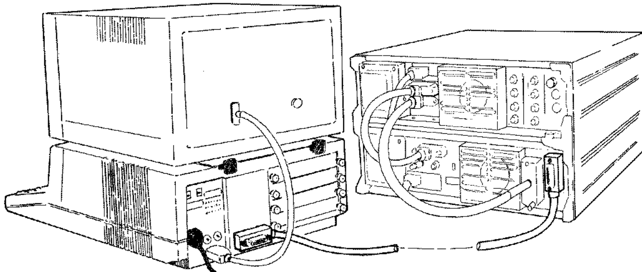
FIGURE 1. SYSTEM CONNECTION
