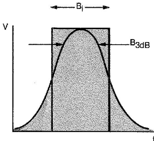
Impulse Bandwidth B_1 is Bandwidth of Rectangular Filter With Same Voltage Response as Actual Filter.
