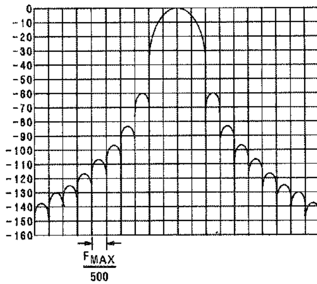
HANNING FILTER WINDOW
