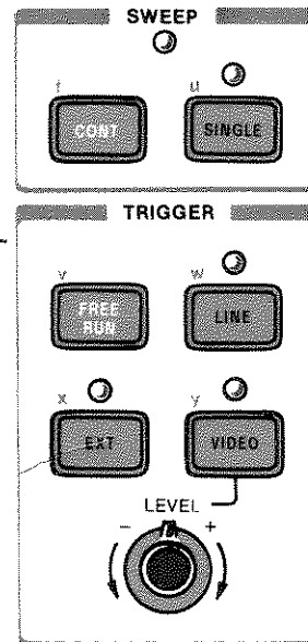
SWEEP and TRIGGER Controls
