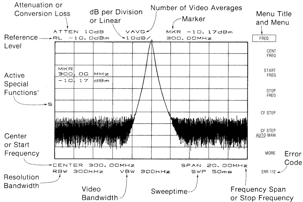
Fig. 1.2. Display annotation.
