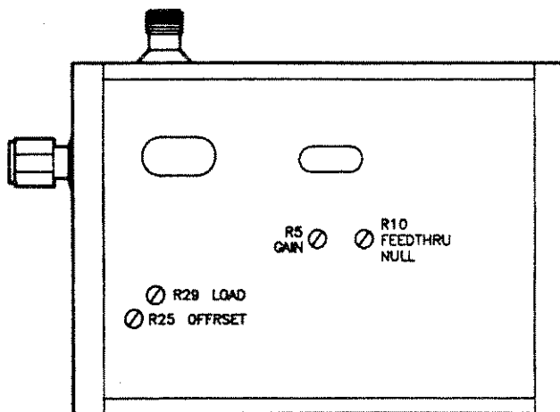
Figure 5-2. Locations of Adjustment Potentiometers
