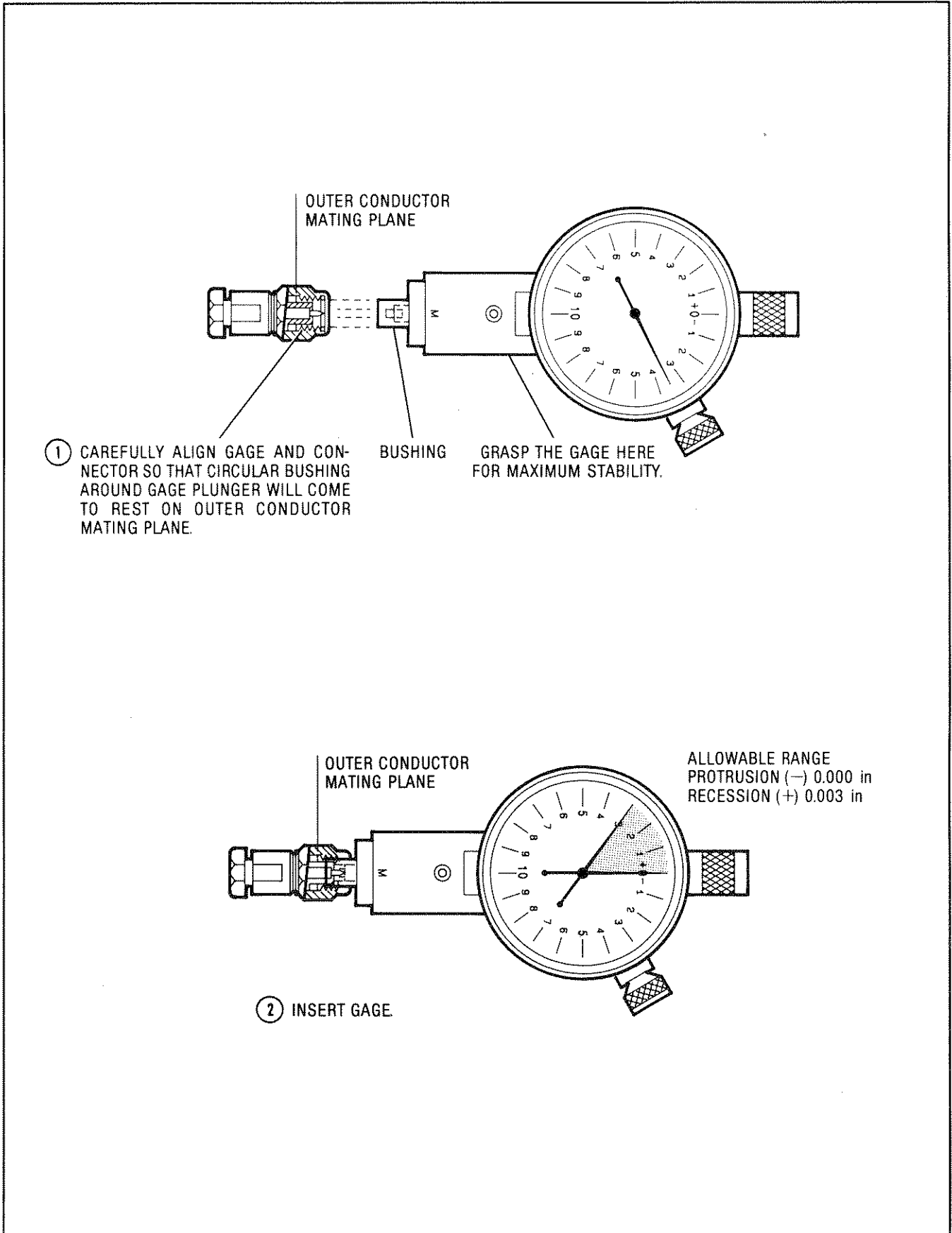
Figure 8-7. Gaging Precision 3.5mm (m) Connector
