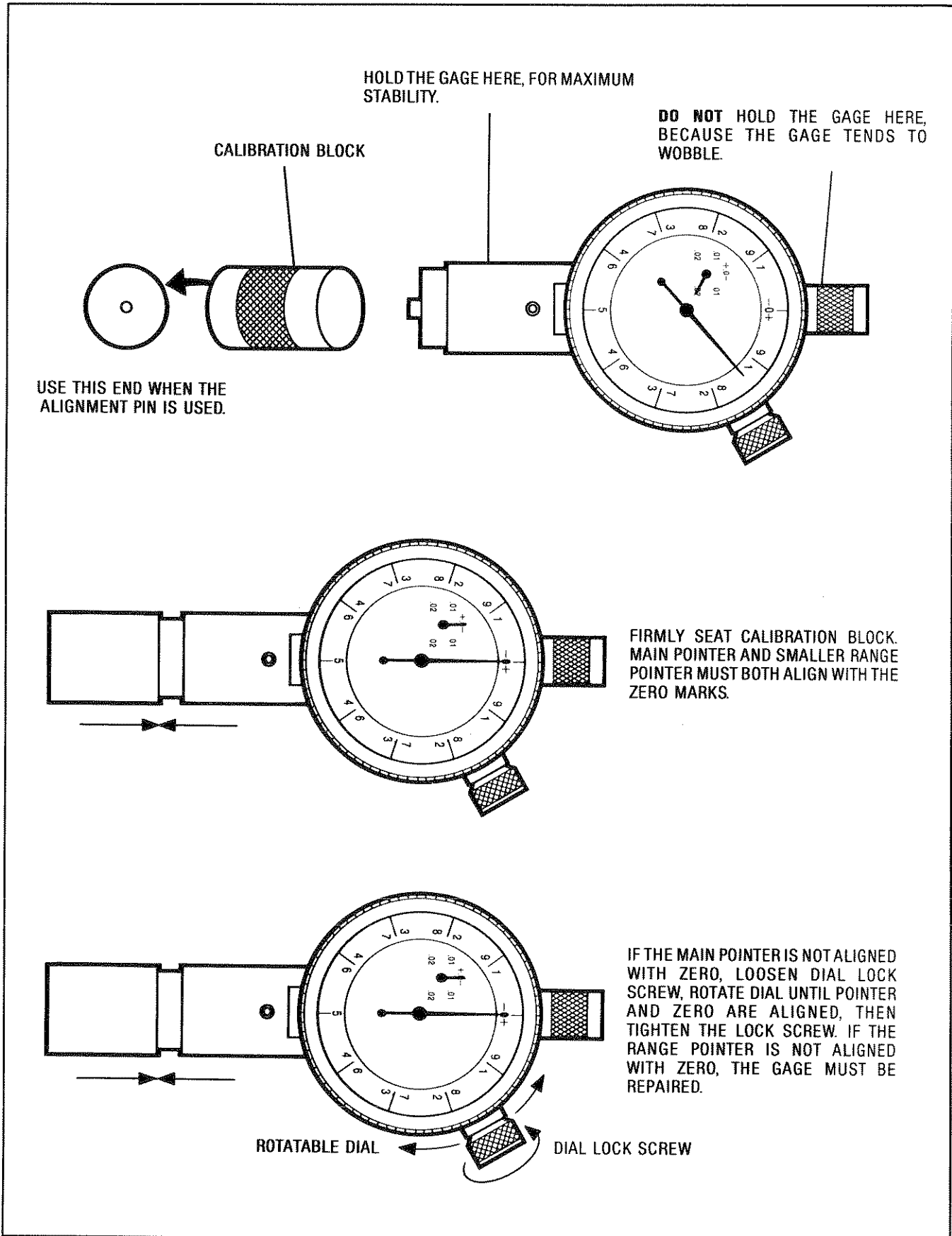
Figure 8-9. Zeroing the APC-7 Gage
