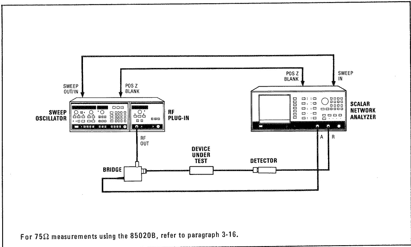
Figure 3-4. Typical Measurement Setup Using 8756A
