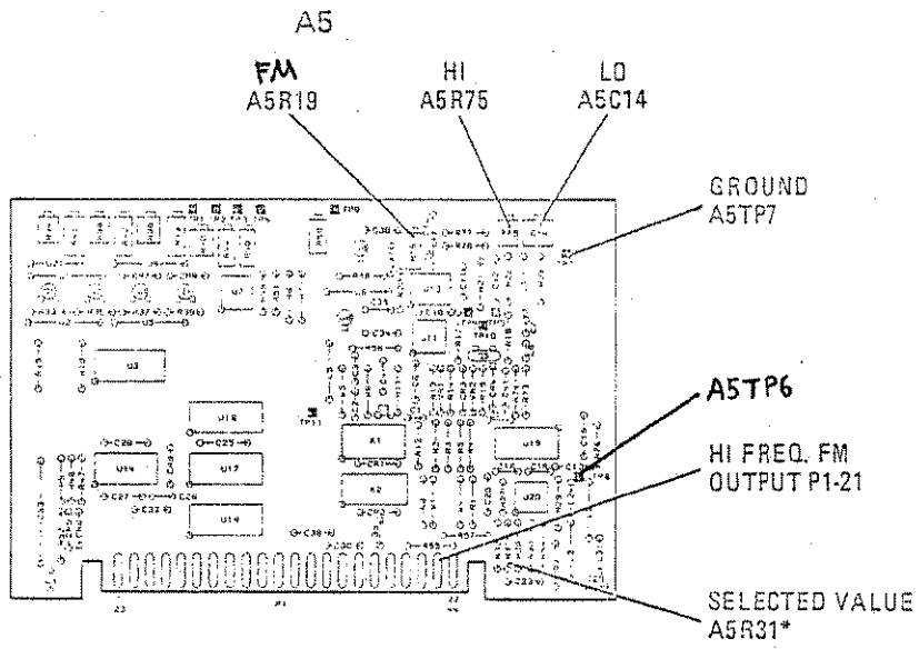
Figure 5-41. Location of A5 FM Driver Adjustments
