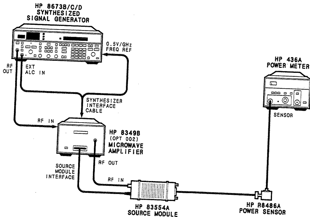
Figure 2-4. System Configuration
