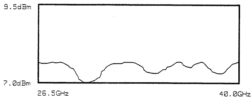
Figure 2-8. Power Flatness Response (26.5 to 40.0 GHz)
