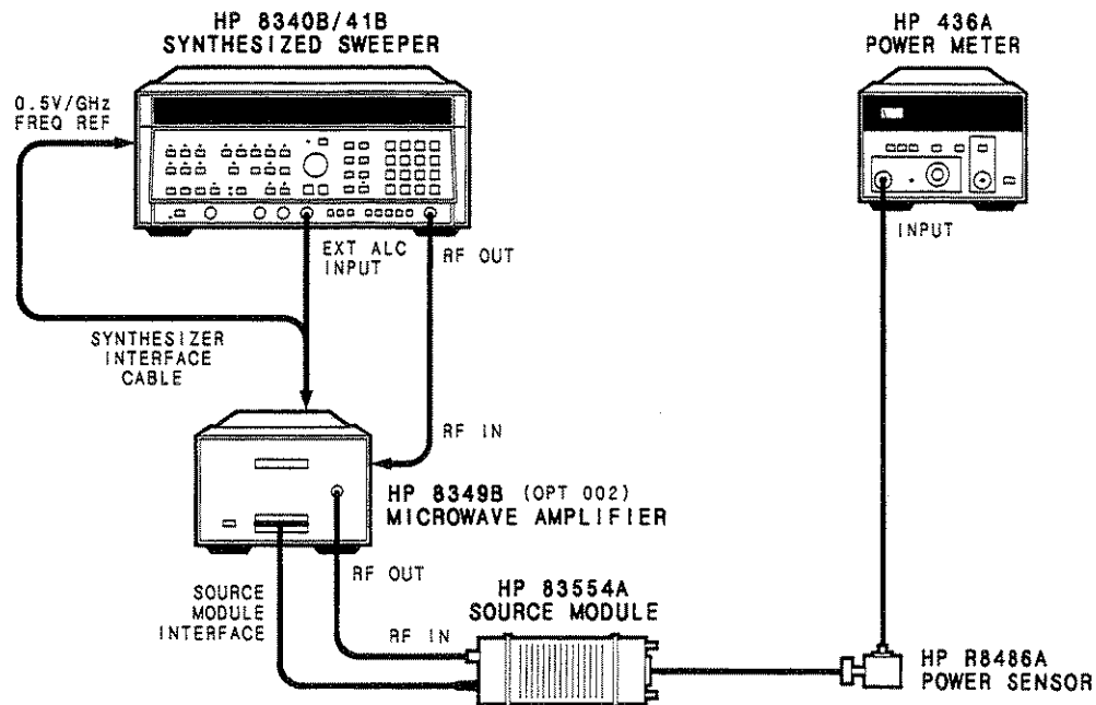
Figure 2-4. System Configuration
