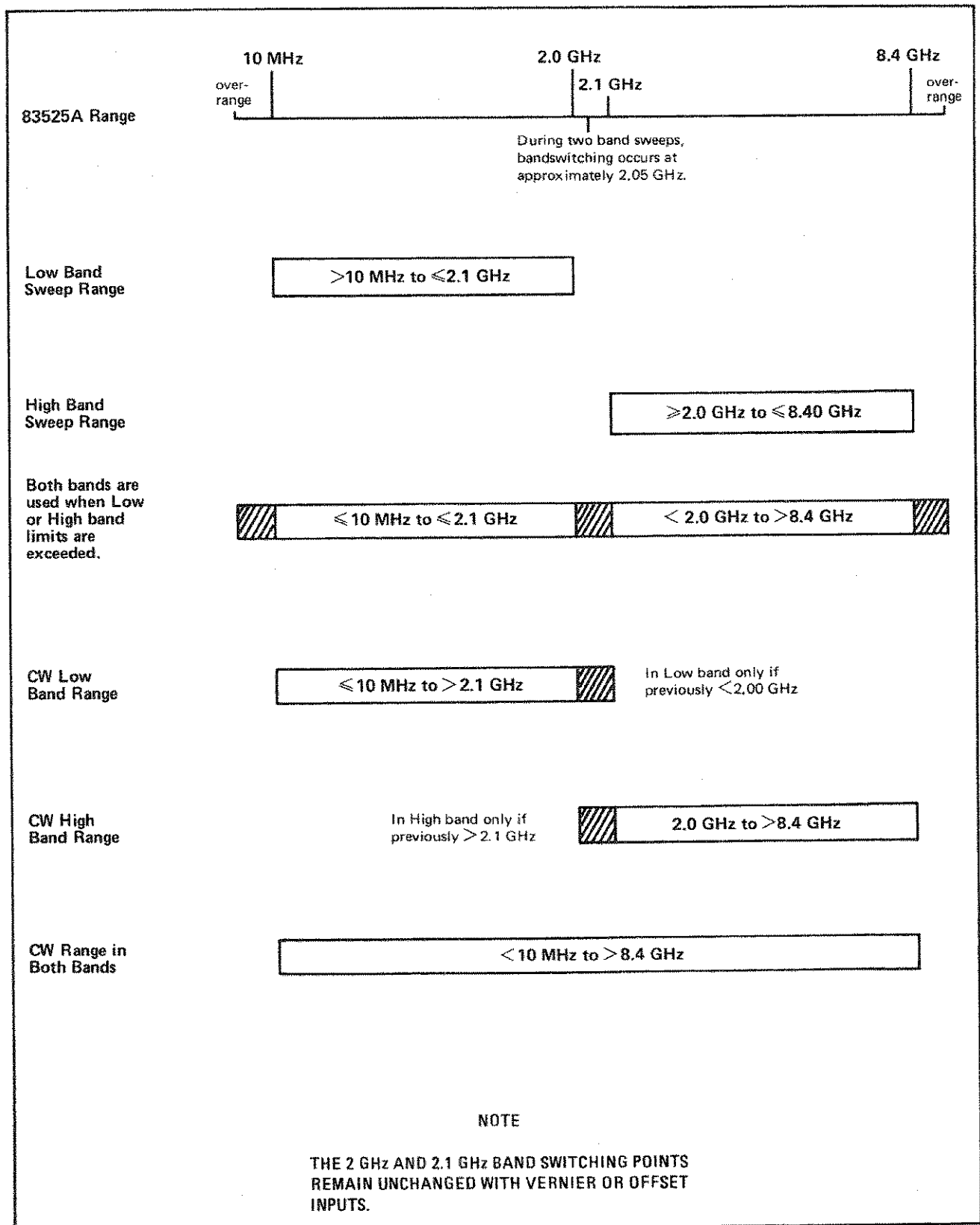
Figure 3-1. Band Switching in CW and Swept Frequency Modes
