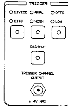
Figure 3-4. TRIGGER controls
