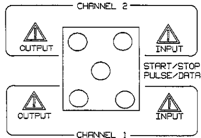
Figure 3-12. Rearpanel signal-connectors
