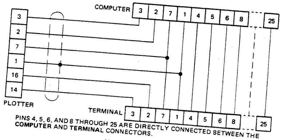
Y-cable Schematic
