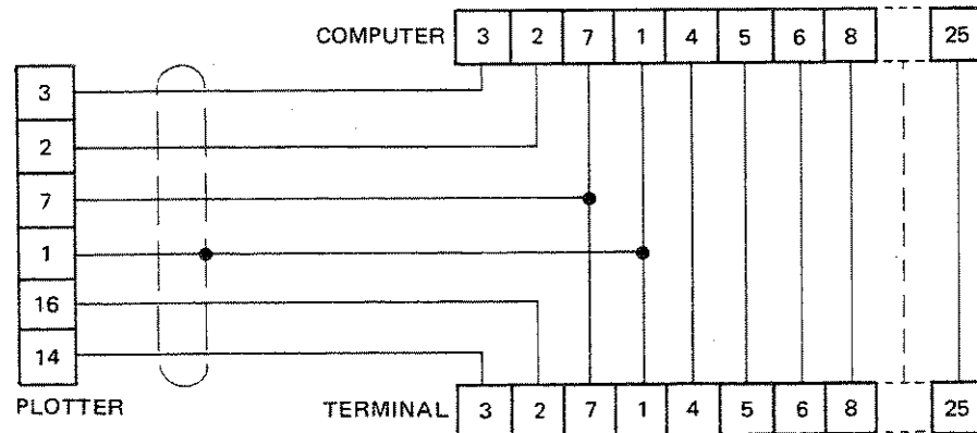
Y-cable Schematic
