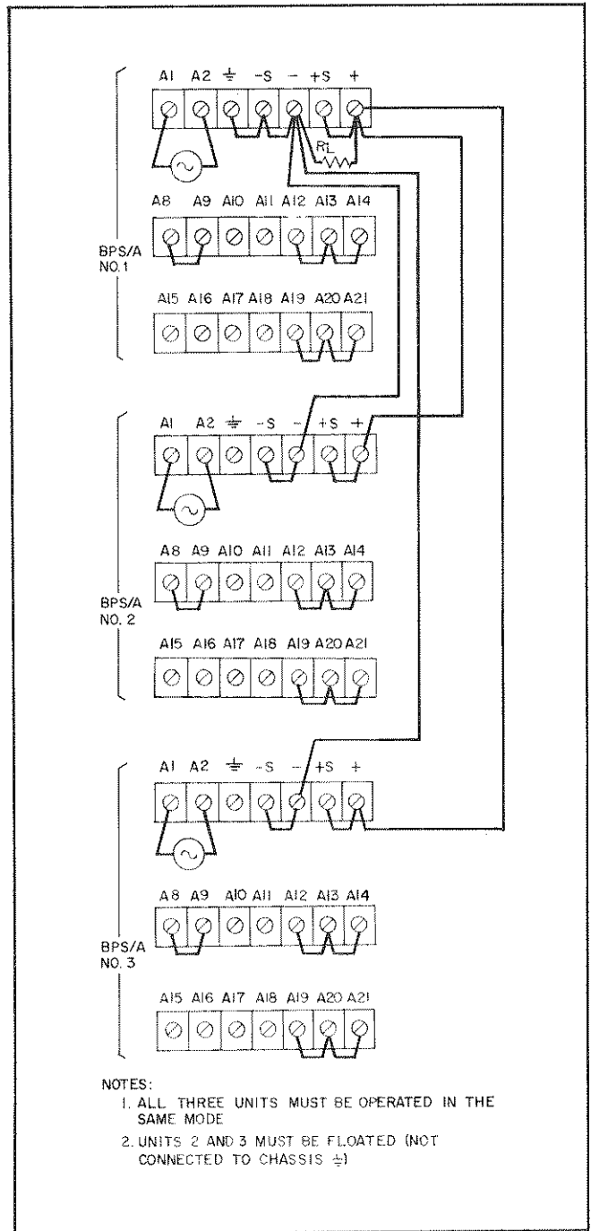
Figure 3-11. Parallel Connections
