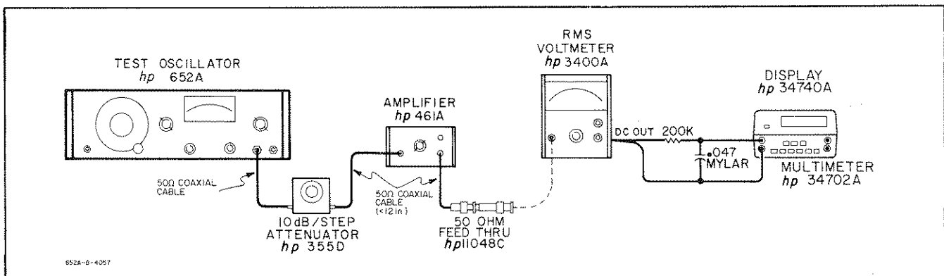
Figure 5-4. Attenuator Test.
