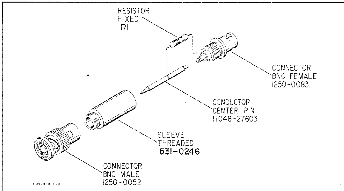
Figure 2. Exploded View.
