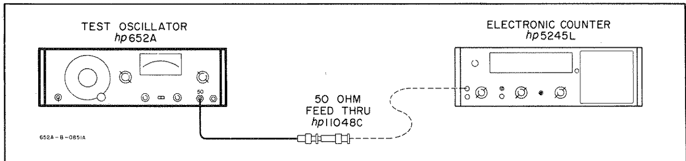
Figure 5-1. Frequency Tests.
