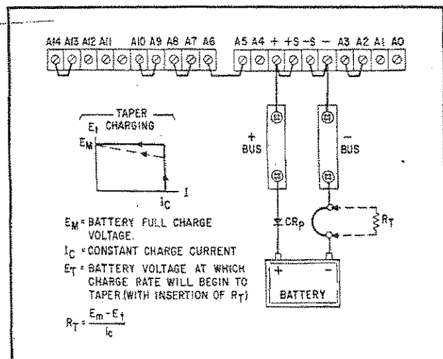
Figure 3-10. Battery Charging
