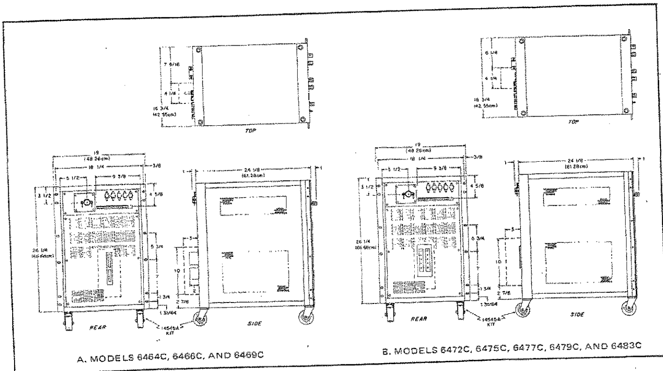
Figure 2-1. Outline Diagram
