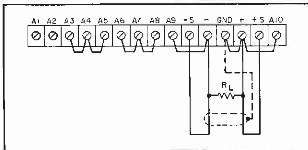
Figure 3-7. Remote Sensing
