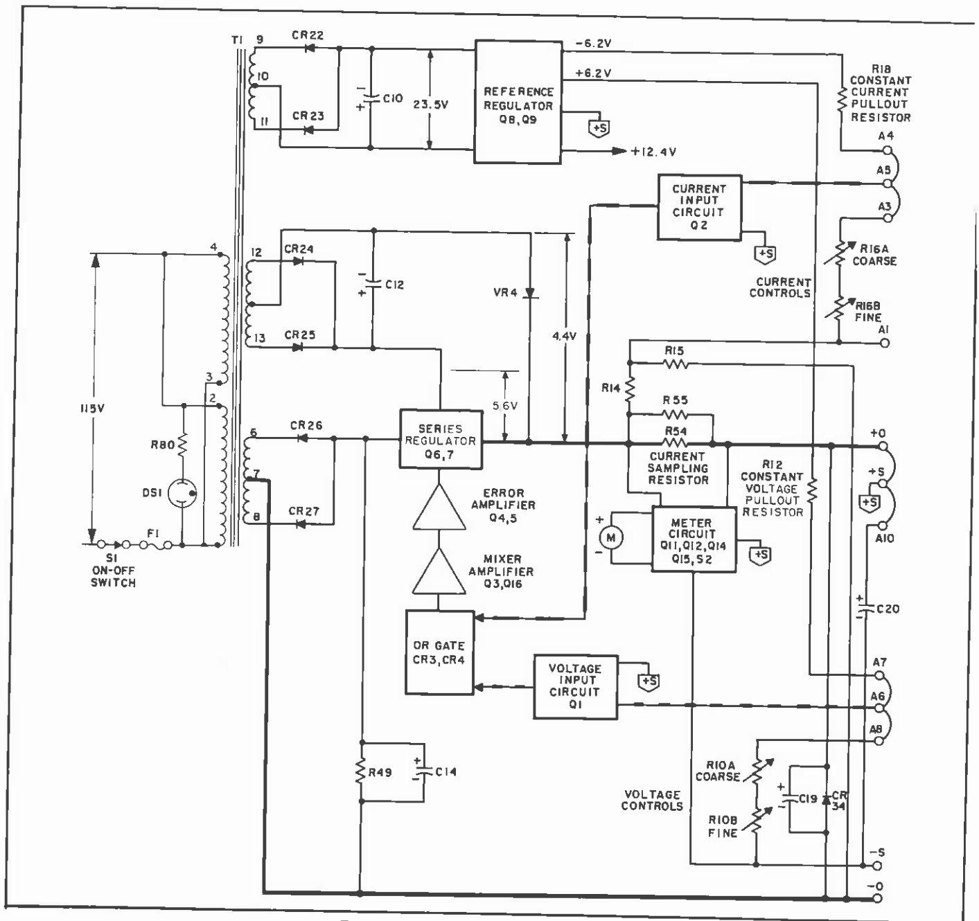
Figure 4-2. Simplified Schematic
