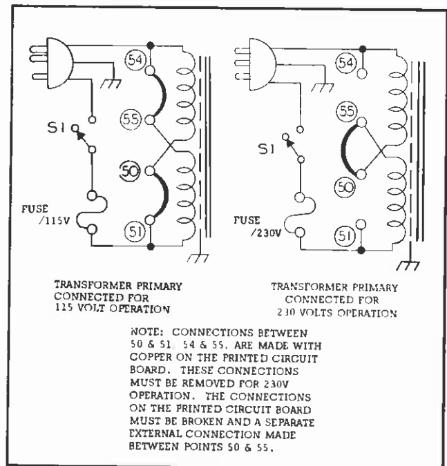
Figure 2-3. Primary Connections
