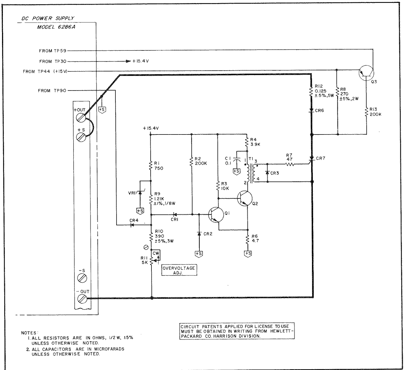
Figure A-1. Model 6286A Overvoltage Protection Crowbar
