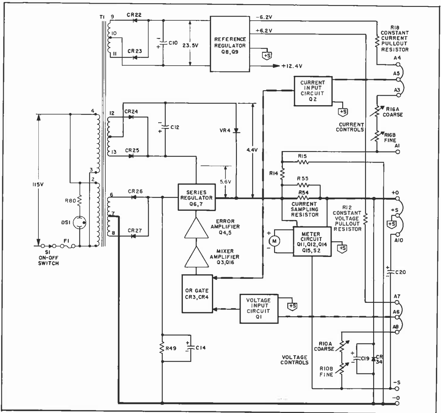
Figure 4-2. Simplified Schematic
