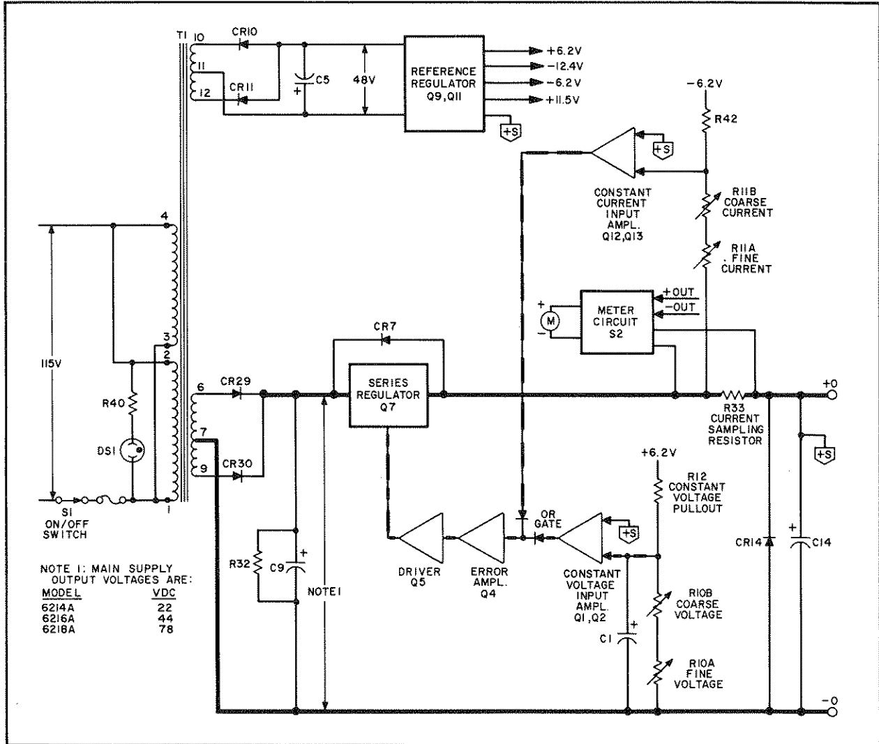
Figure 4-1. Block Diagram
