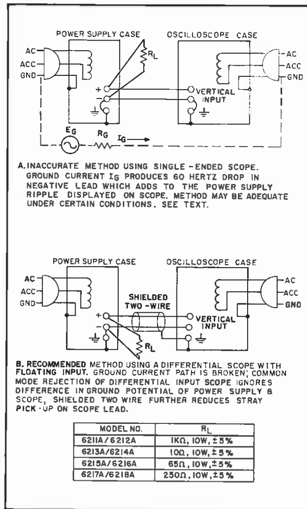
Figure 5-6. Ripple and Noise, Test Setup
