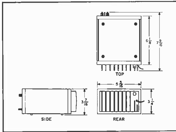
Figure 2-1. Outline Diagram
