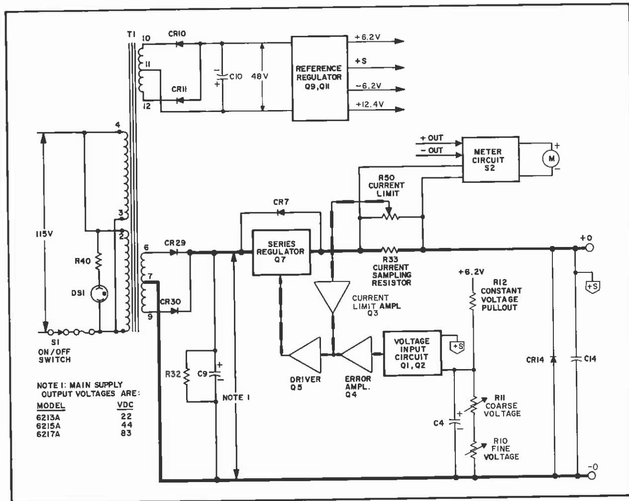
Figure 4-1. Simplified Schematic
