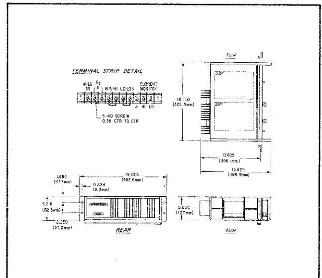
Figure 2-1. Outline Diagram
