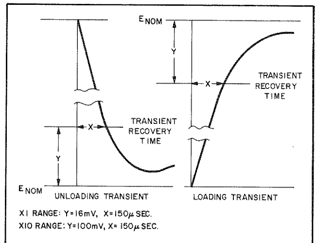
Figure 5-6. Transient Recovery Time, Waveforms
