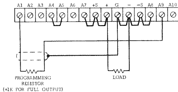
Figure 3-5. Remote Resistance Programming (Current Limit)
