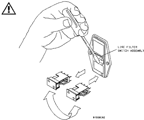
Removing and installing the fuse module.
