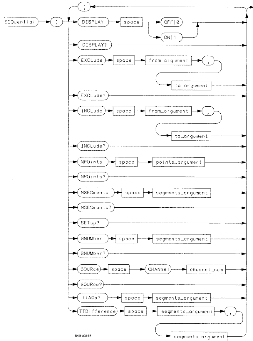
Sequential Subsystem Commands Syntax Diagram
