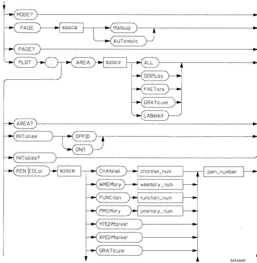
Hardcopy Subsystem Commands Syntax Diagram (continued)
