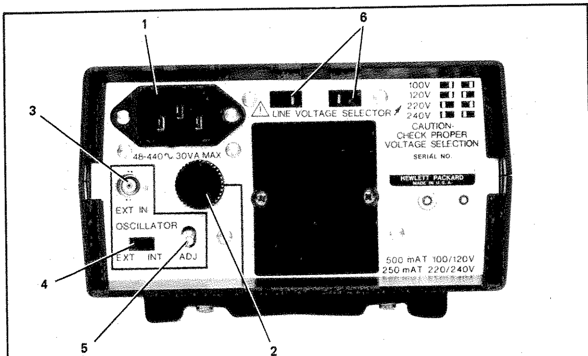
STANDARD INSTRUMENT REAR VIEW
