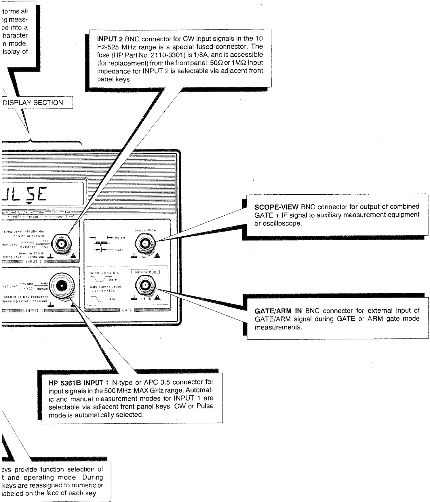
Figure 3-2. Front Panel Features
