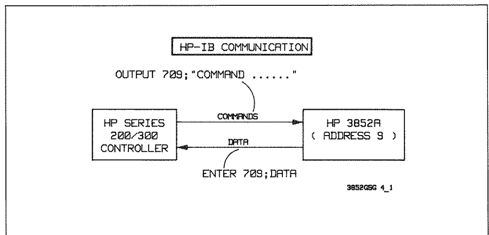
Figure 4-1. HP-IB Communication
