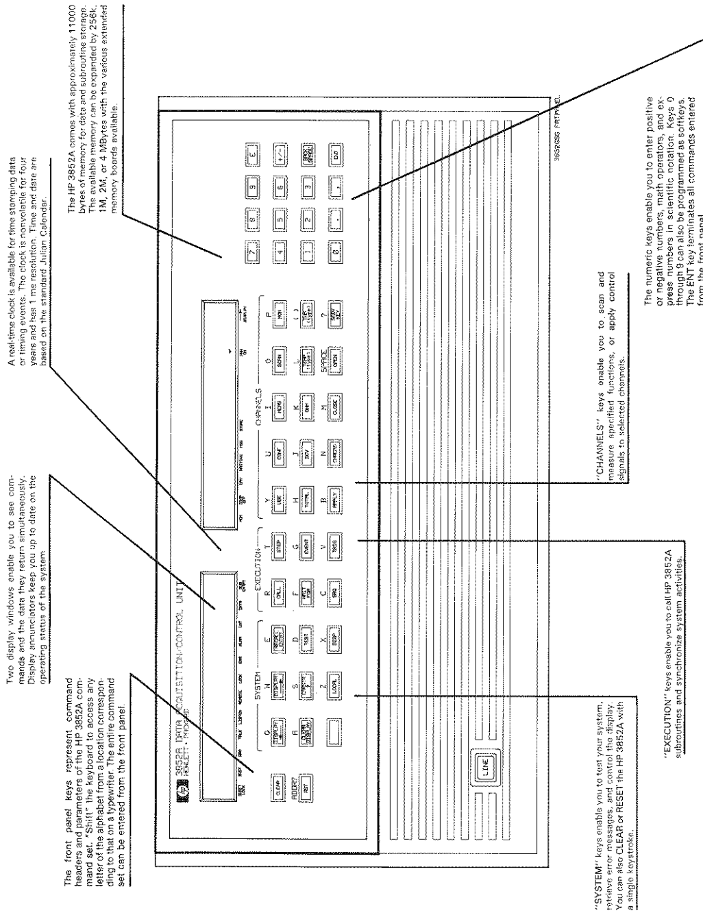
Figure 1-2. HP 3852A Front Panel
