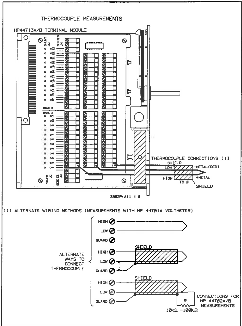
Figure 4-5. HP 44713A/B Thermocouple Connections
