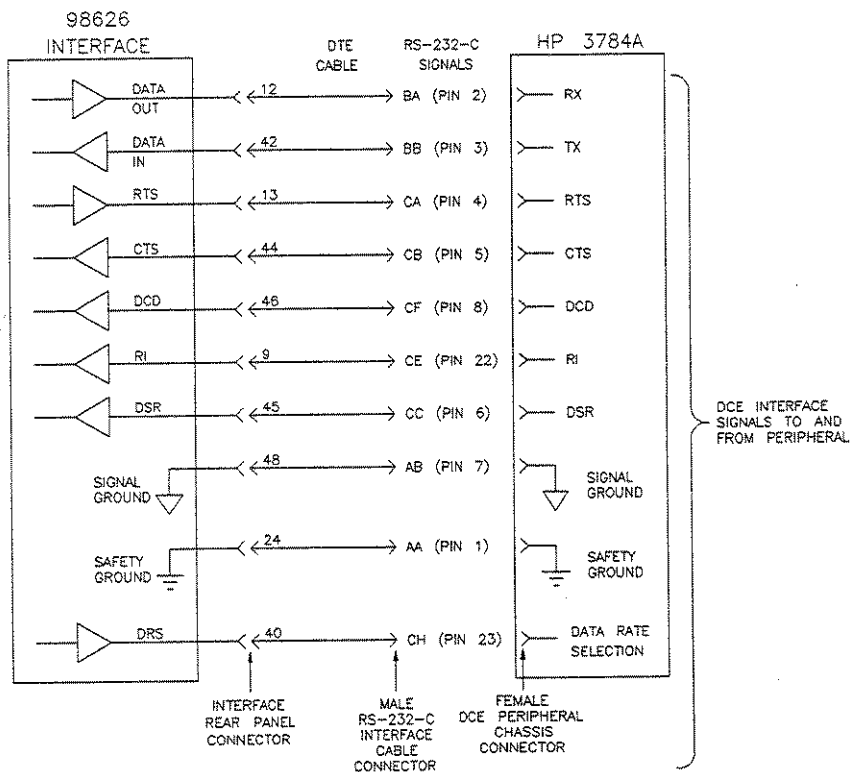
Figure 2-4 DTE Cable Interconnection Diagram
