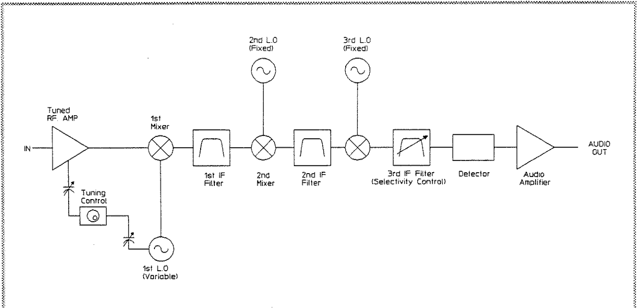
Typical Superheterodyne Communications Radio Receiver
